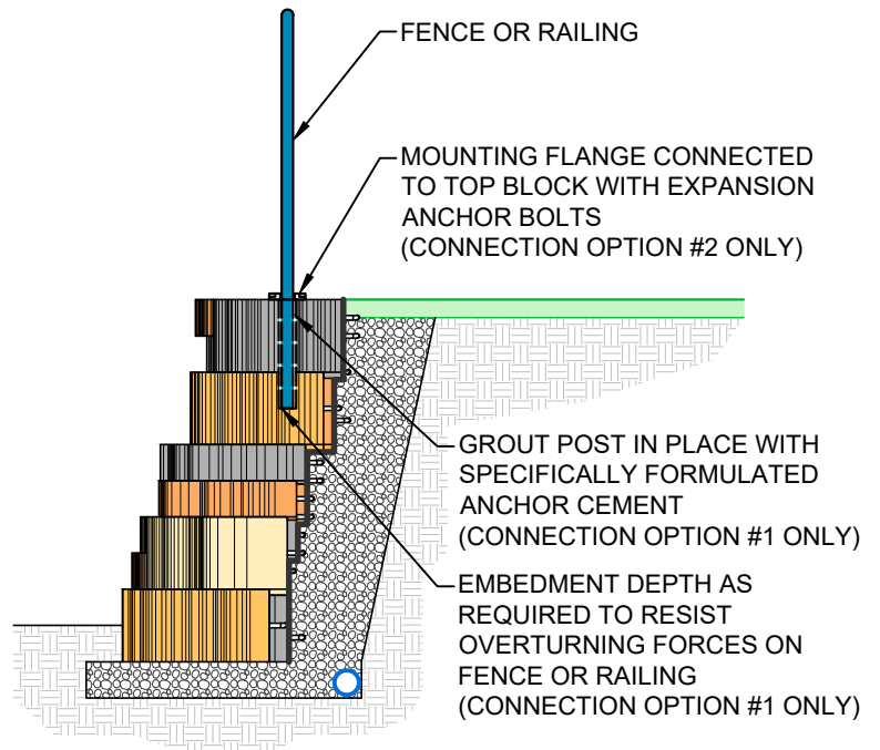
SIDE VIEW (NO SCALE)
