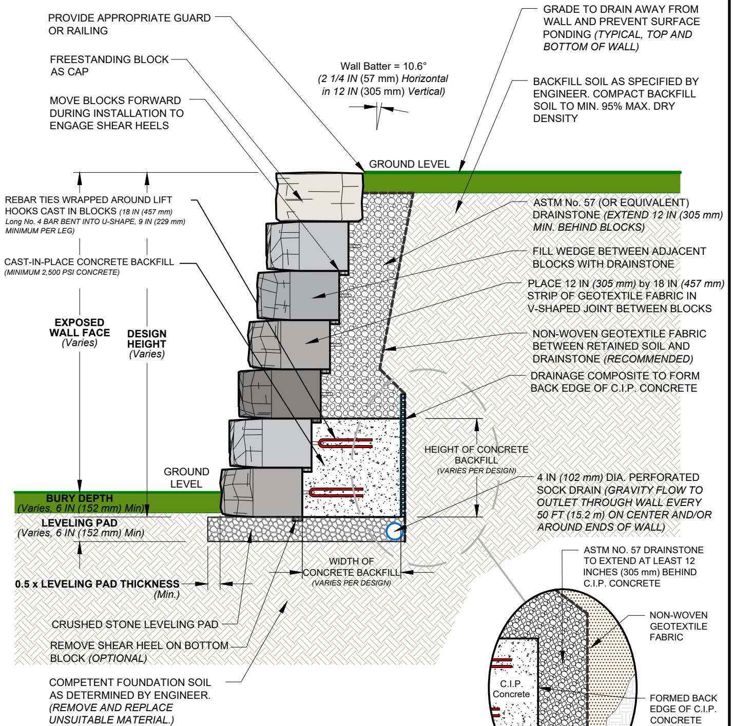
TYPICAL SECTION (NO SCALE)
