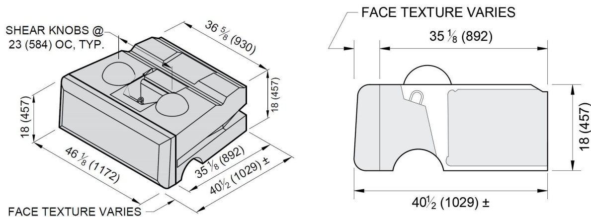
Figure 2 - R-41PC Block and Cross Sectional Depiction
