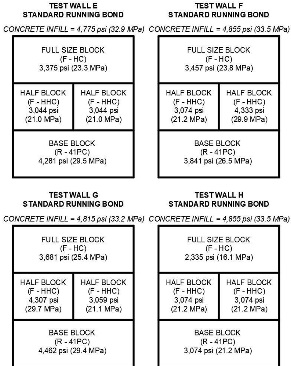
Figure 4 - Concrete Compressive Strengths (looking from the front of the wall sample)
