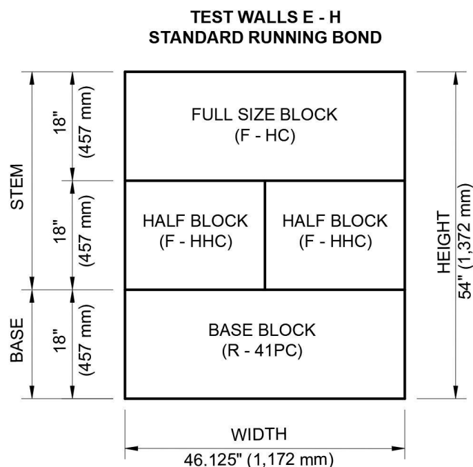
Figure 5 - Test Block Layout (looking from the front of the wall sample)
