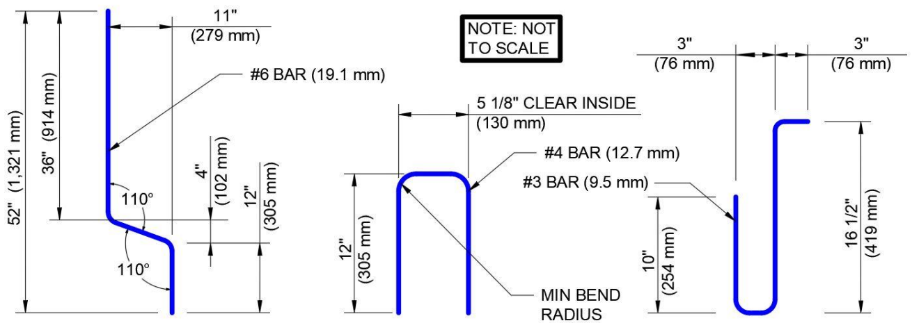
Figure 7 - Rebar Details. Bent Reinforcement Bars, and U-Shaped stirrups, and hook.
