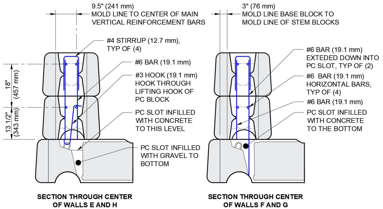
Figure 6 - Wall Cross Sections
