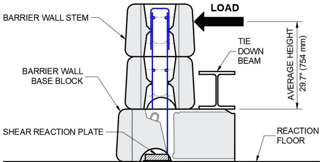
Figure 11 - Test Set-up
