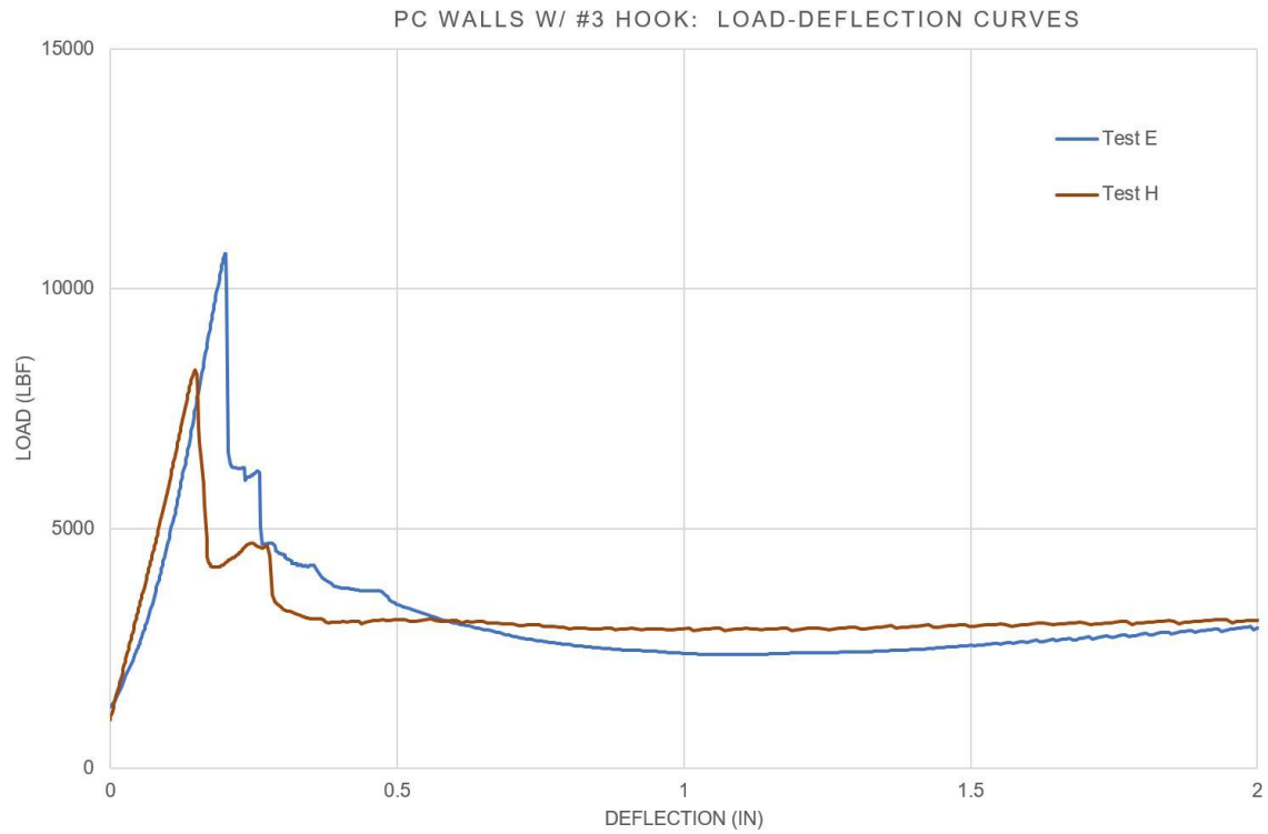
Figure 14 - Test Results by Wall Type (Tests E and H)
