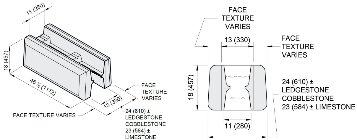
Figure 3 - F-HC Block and Cross Sectional Depiction
