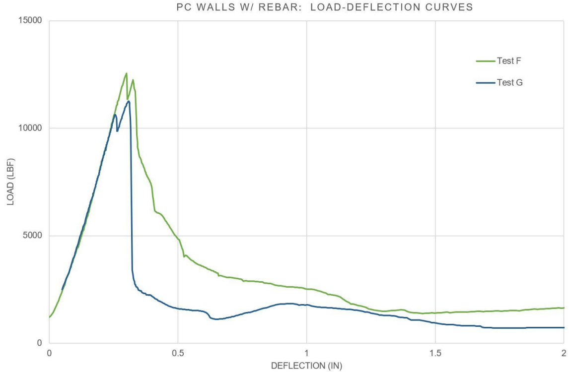
Figure 15 - Test Results by Wall Type (Tests F and G)
