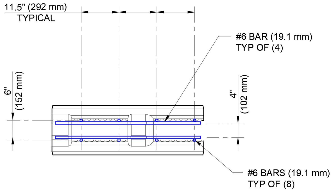
Figure 8 - Top View of Walls E and H (#3 HOOK)
