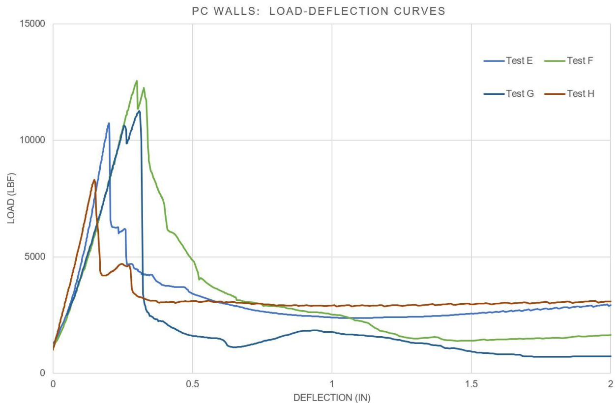
Figure 13 - Test Results (All four tests)
