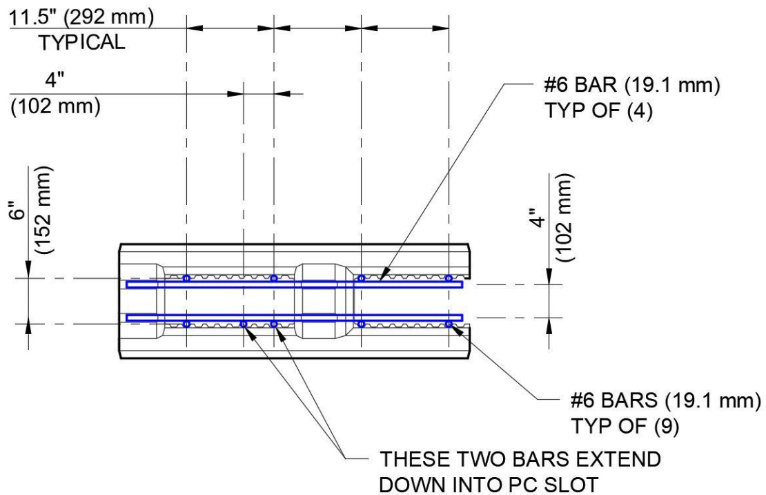
Figure 9 - Top View of Walls F and G (Rebar)
