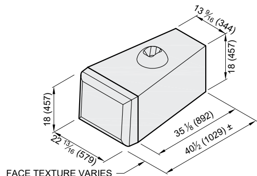
HALF BOTTOM
