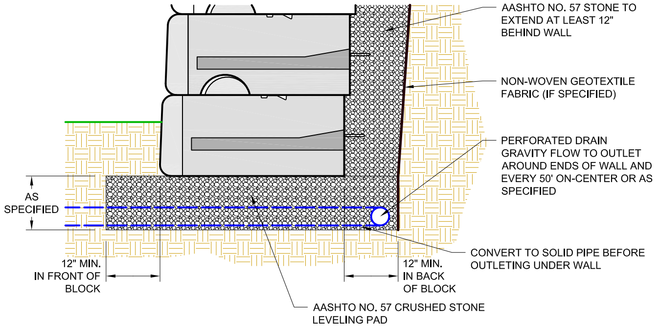
OPEN-GRADED CRUSHED STONE LEVELING PAD
