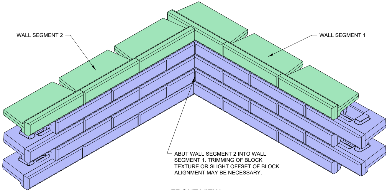
FRONT VIEW
