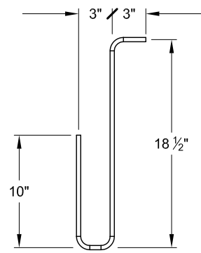
BEND DETAIL NO. 3 REBAR HOOKS
