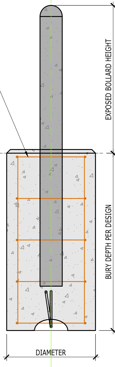
VERTICAL SECTION
