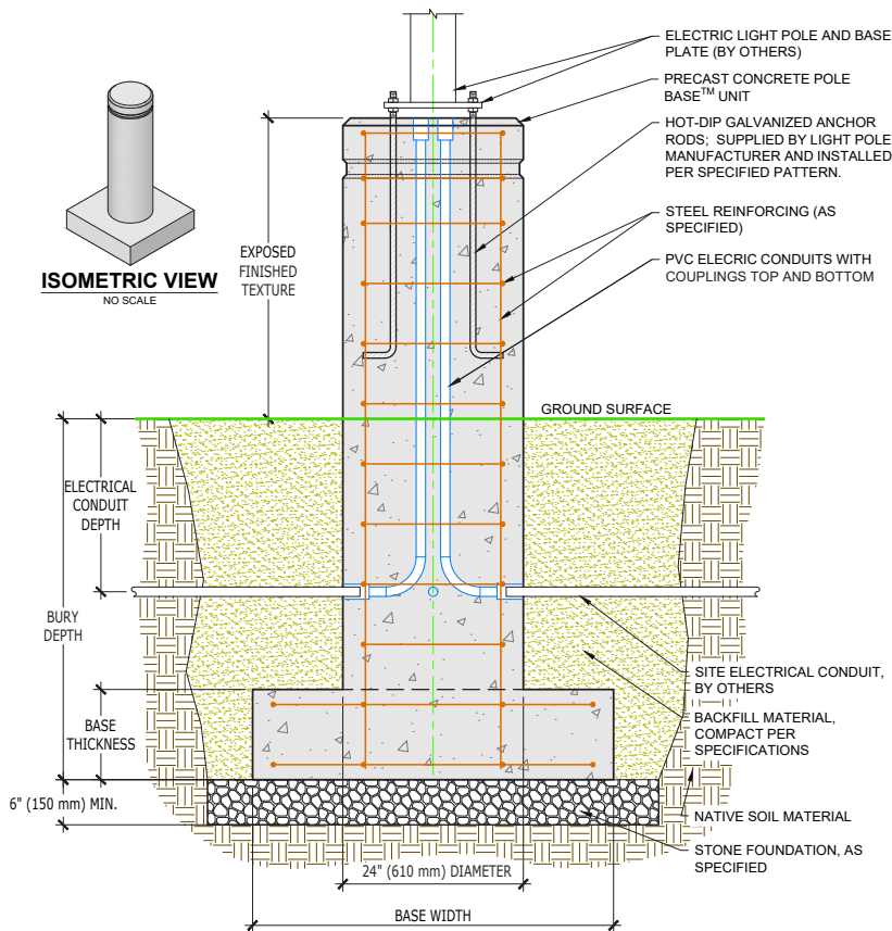
24 inch (610 mm) Diameter Round Pole Base Spread Footing
