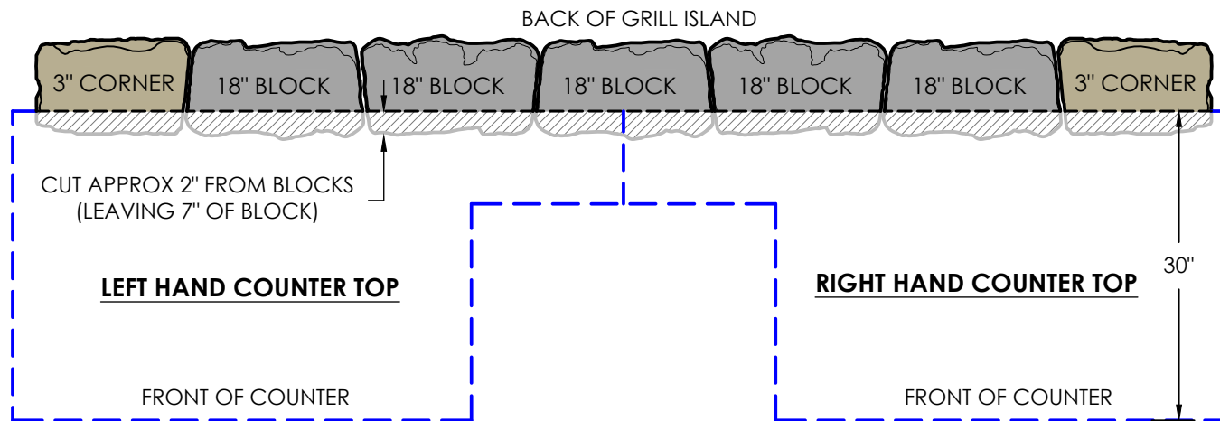
BLOCKS CUTS AT BACK OF COUNTER (LOOKING FROM ABOVE)
