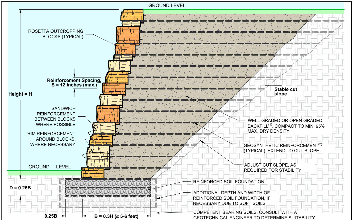
TYPICAL SECTION (NO SCALE)
