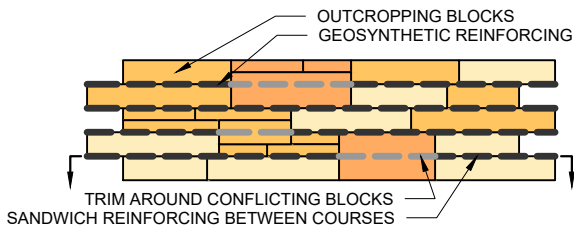
CONNECTION ELEVATION (NO SCALE)
