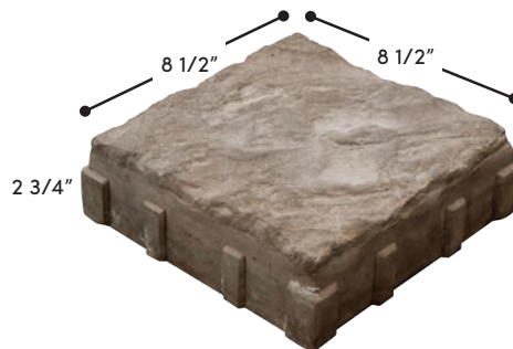
9 X 9 PAVER
