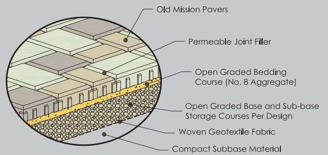
PERMEABLE PAVER CROSS-SECTION
