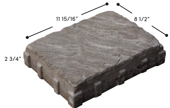
9 X 12 PAVER
