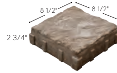
9 X 9 PAVER
