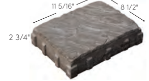
9 X 12 PAVER
